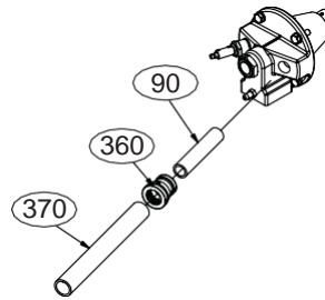
3/4" EXTENDED UV SCANNER OPTION
