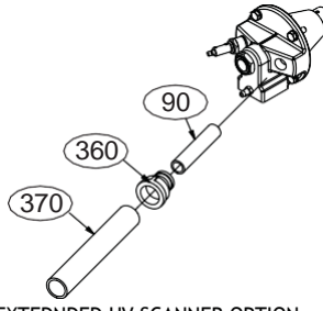
1" EXTENDED UV SCANNER OPTION
