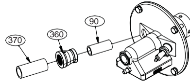
3/4" UV SCANNER OPTION
