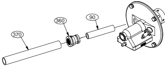
EXTENDED 3/4" UV SCANNER OPTION
