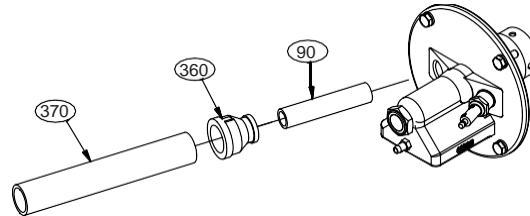
EXTENDED 1" UV SCANNER OPTION
