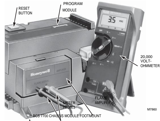
Fig. 19. Measuring voltage flame signal with BCS 7700 (currently obsolete) controls.
