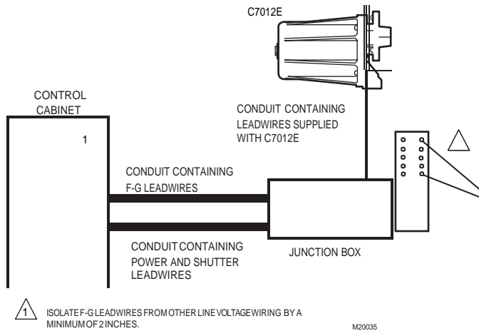
Fig. 9. Splicing leadwires in a junction box.
