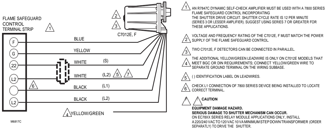
Fig. 16. Wiring diagram for C7012E,F Detectors with 7800 SERIES Flame Safeguard Controls with shutter drive circuitry.
