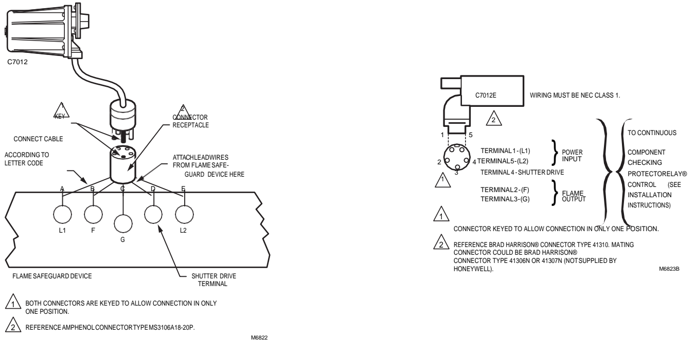
Fig. 17. Wiring connection for C7012E1161 or C7012E1278.
