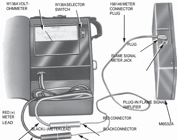
Fig. 18. Measuring microamp flame signal.
