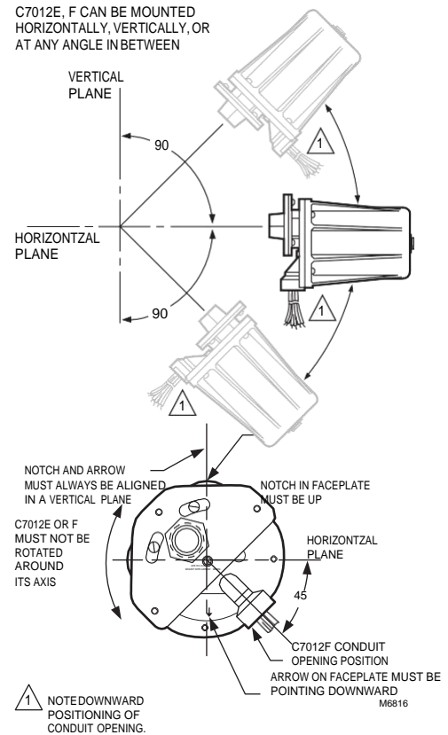
Fig. 6. C7012E,F mounting positions.
