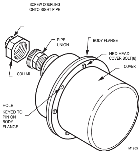
Fig. 8. Mounting C7012C or F Detector.
