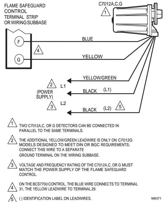
Fig. 10. Wiring diagram for C7012A,C, or G Detectors with rectification type, flame safeguard primary and programming controls.
