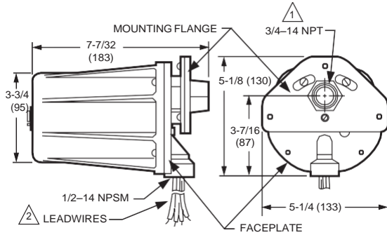
C7061A1046: 1 INCH NPT
