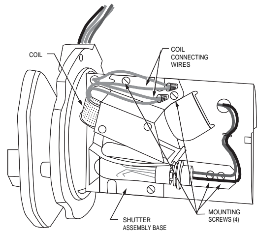
Fig. 13. Replacing coil and shutter assembly.
