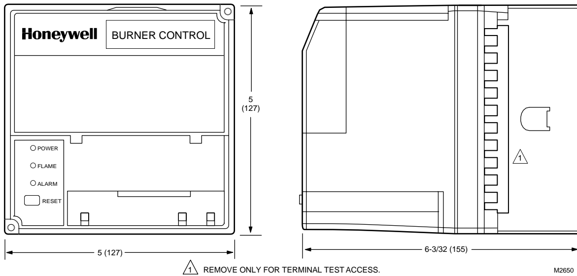
Fig. 1. Mounting dimensions of EC7823IRM7823 Relay Module and Q7800A,B Subbase in in. (mm).
