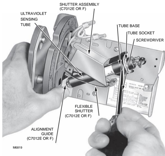
Fig. 12. Replacing ultraviolet radiation sensing tube.
