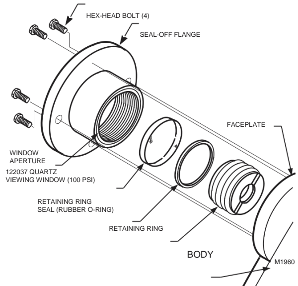
Fig. 15. Replacing quartz viewing window on C7024F.
