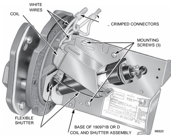
Fig. 13. Replacing coil and shutter assembly on C7024E,F.
