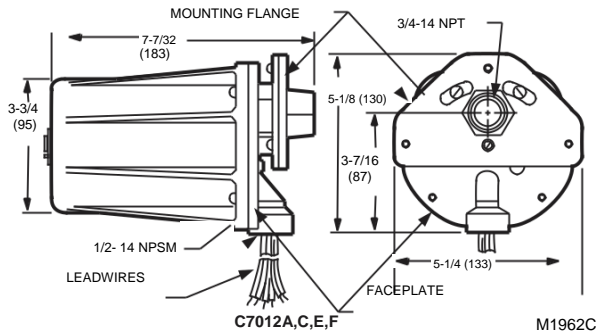
Fig. 1. Dimensions of C7024E in in. (mm).
