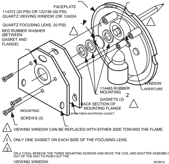
Fig. 14. Replacing quartz viewing window or focusing lens on C7024E.
