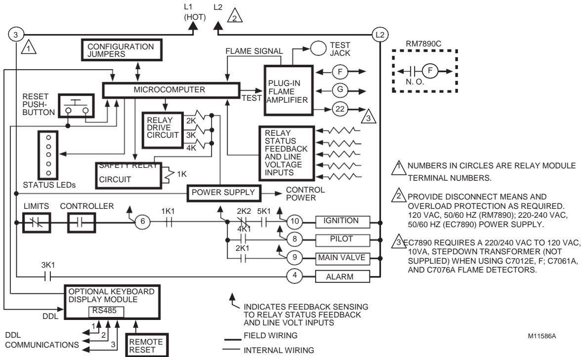
Fig. 1. Internal block diagram of the RM/EC7890.
