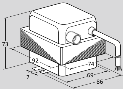
TZI 5-15/100, TZI 7-25/20
