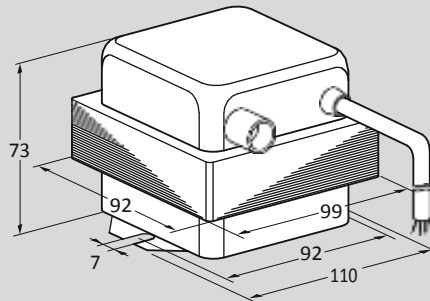
TZI 7,5-12/100, TZI 7,5-20/33
