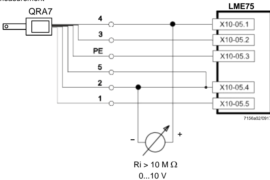
Connection diagram with flame signal measurement
