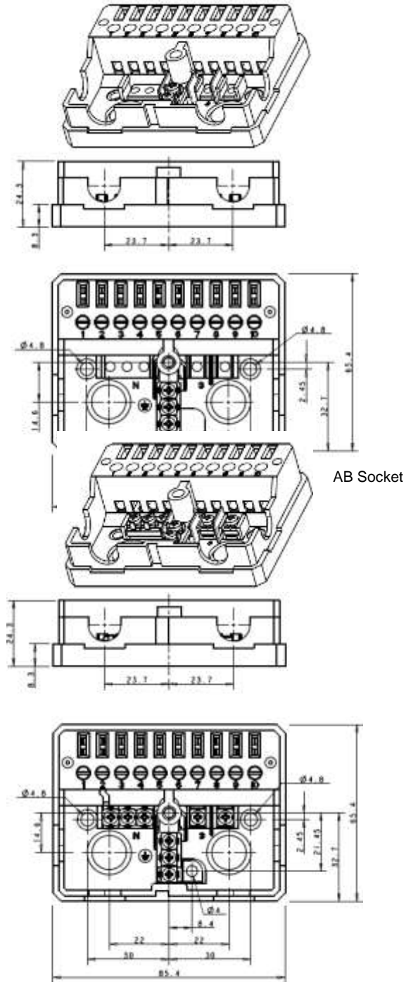
N Socket Fig.2
