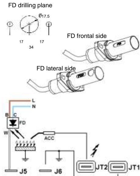
Fig.5a-Type, fixing systems and connections of FD s sensors
