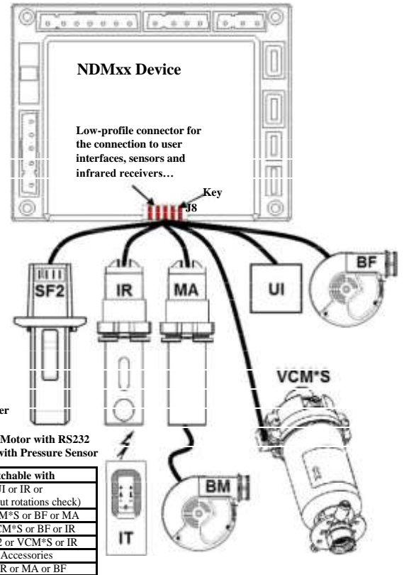
Fig. 6.c – Connectivity of J8 Gate
