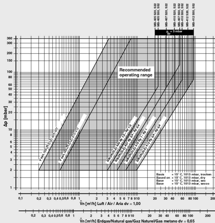
Volumetric flow pressure loss characteristics in regulated state with fine-mesh sieve
