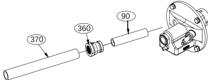
EXTENDED 3/4" UV SCANNER OPTION
