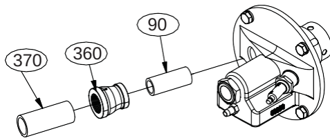
3/4" UV SCANNER OPTION
