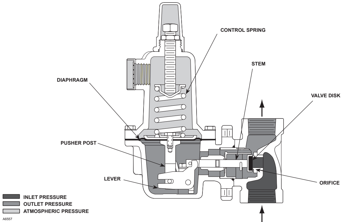
Figure 2. Type 627 Operational Schematic
