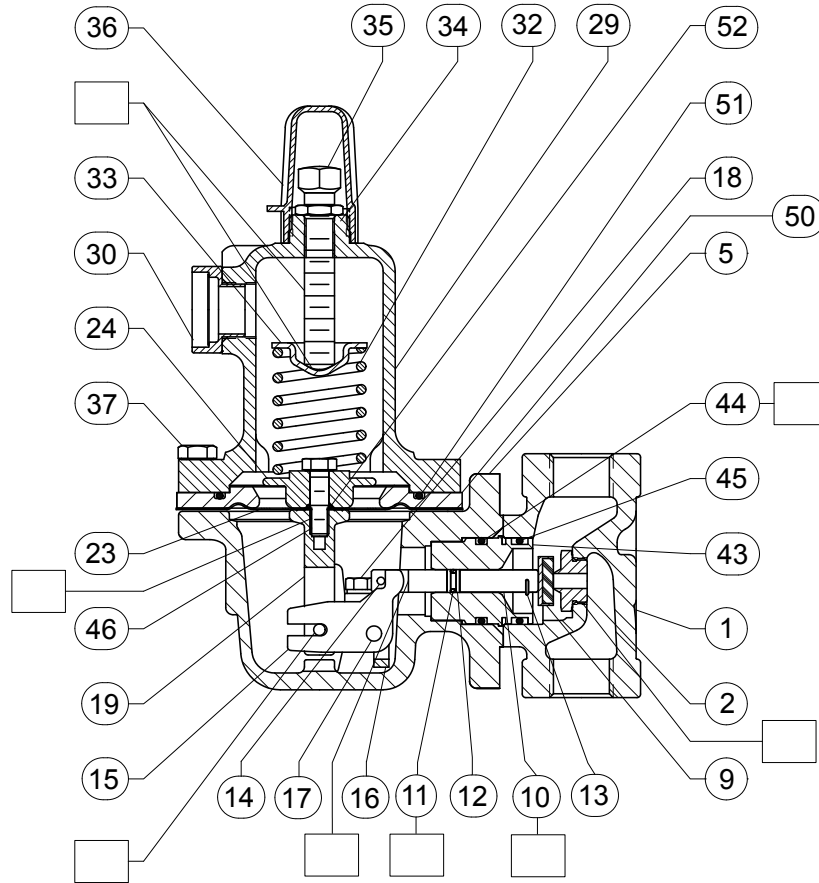
Figure 13. Type 627HM Regulator Assembly
