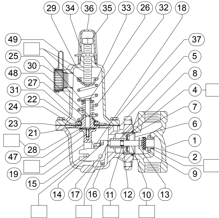
Figure 8. Type 627R Regulator Assembly
