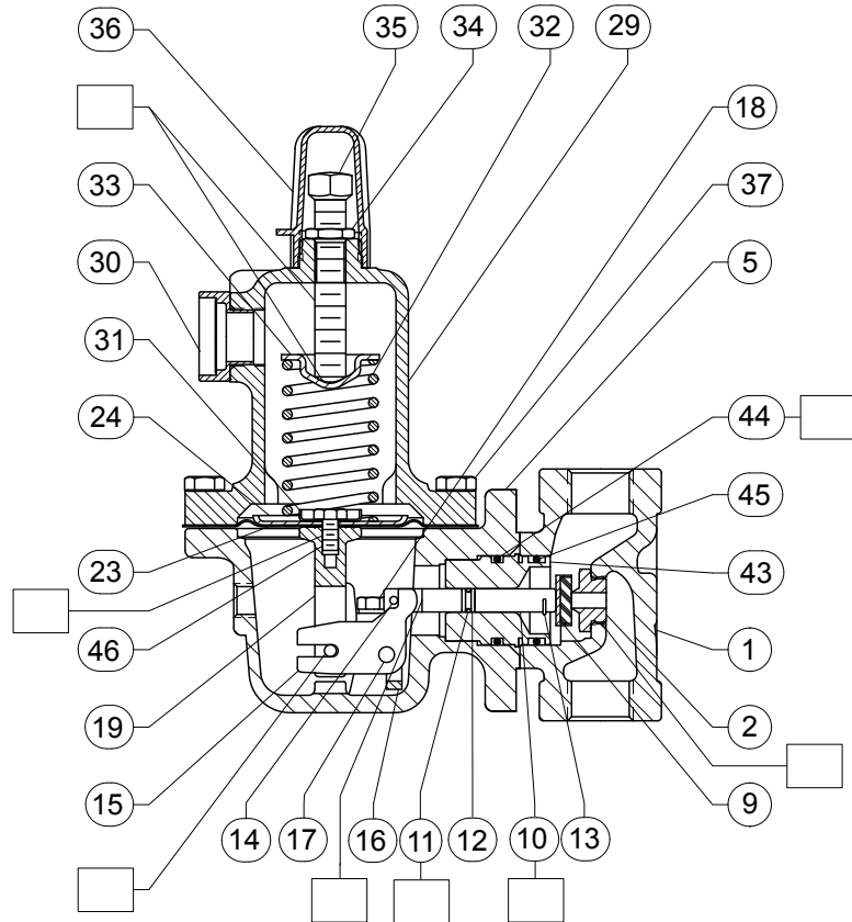
Figure 10. Type 627M Regulator Assembly
