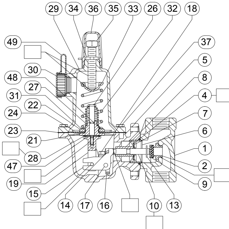
Figure 9. Type 627LR Regulator Assembly
