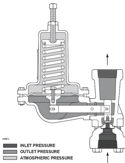
Figure 3. Type 630 Operational Schematic
