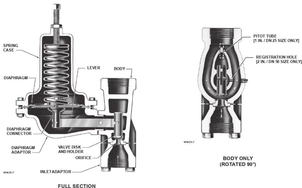
Figure 2. Type 630 Sectional Views
