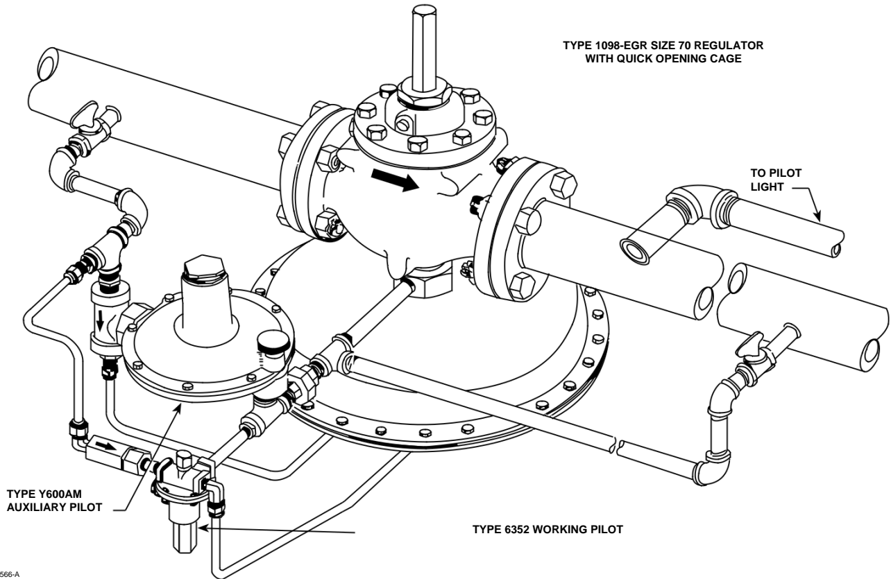
Figure 5. Boiler Fuel Configuration
