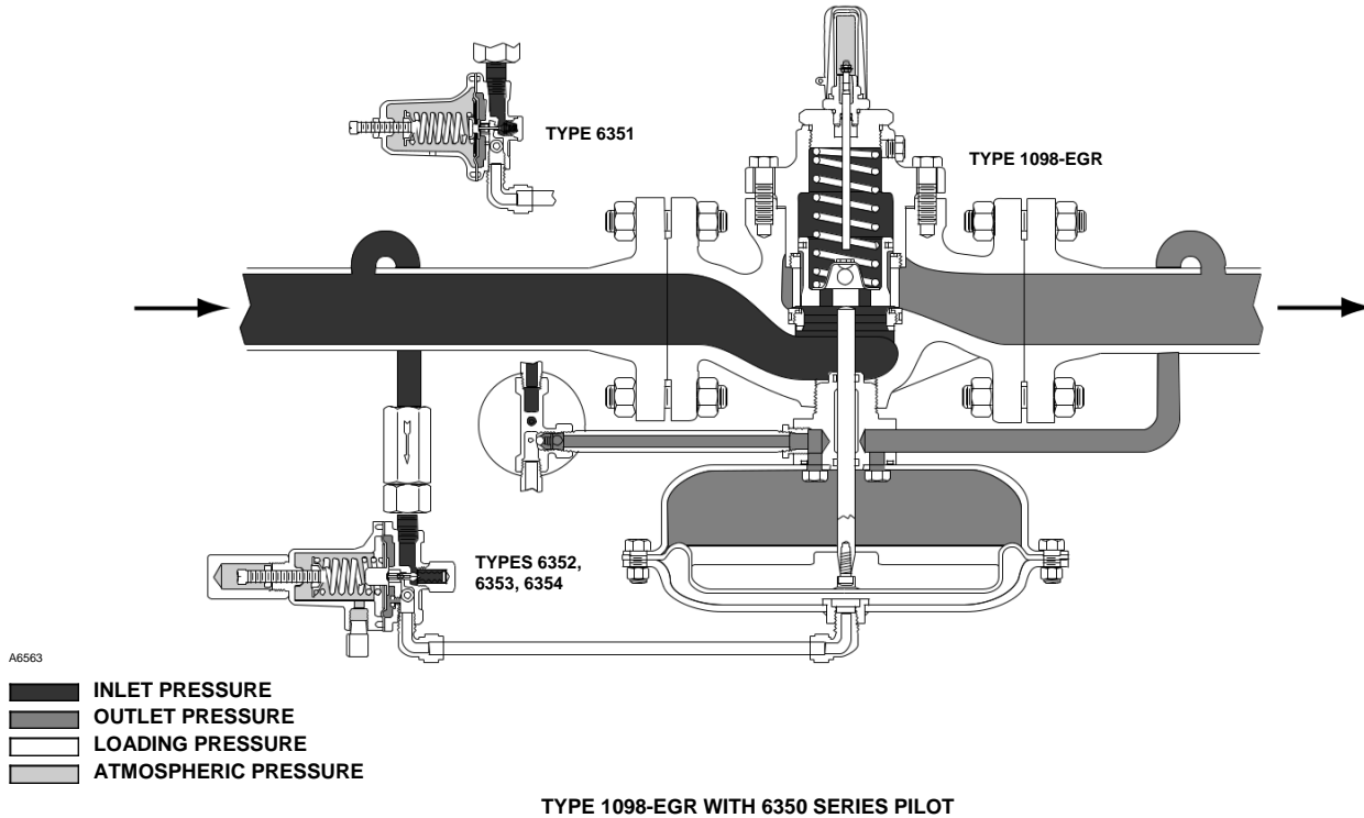
Figure 2. Operational Schematics
