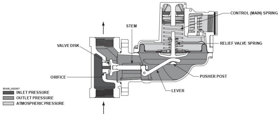
Figure 2. Type HSR Pressure Regulator Operational Schematic
