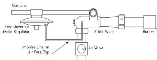
Figure 3c. Typical ratio control system with zero governor ratio regulator cross-connected to the air pressure.
