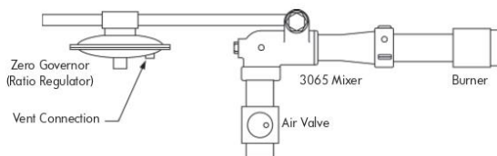
Figure 3. Typical ratio control system with zero governor ratio regulator
