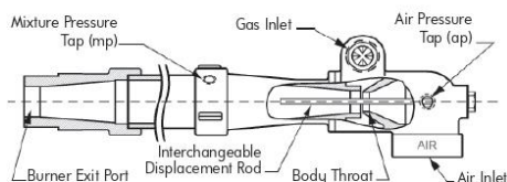
Figure 2. Typical 3065 Mixer & Premix Burner
