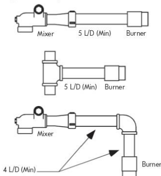
Figure 5. Minimum recommended straight pipe runs
