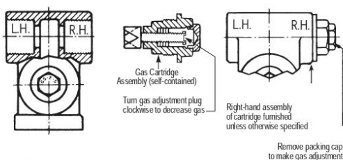
Figure 4. Gas Cartridge detail of 3065 Aspirator Mixer
