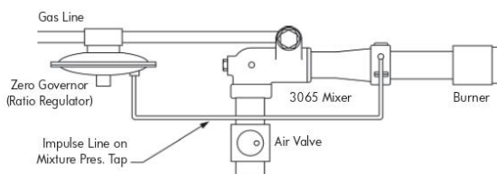
Figure 3b. Typical ratio control system with zero governor ratio regulator cross-connected to the mixture pressure.
