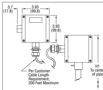
Remote Mounted with Junction Box (EN4)
