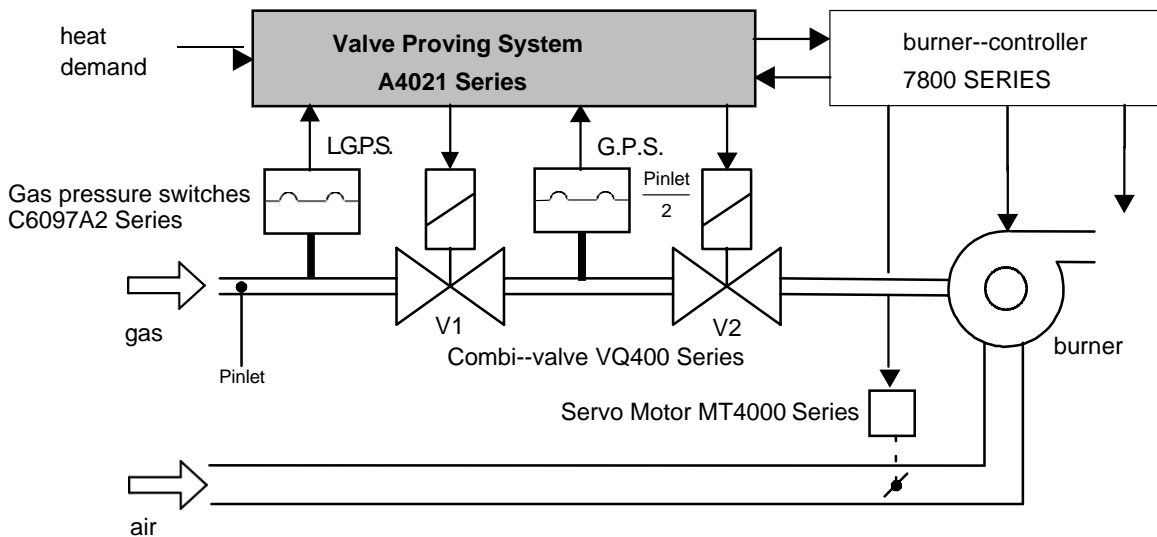
Fig. 4. System set-up .
