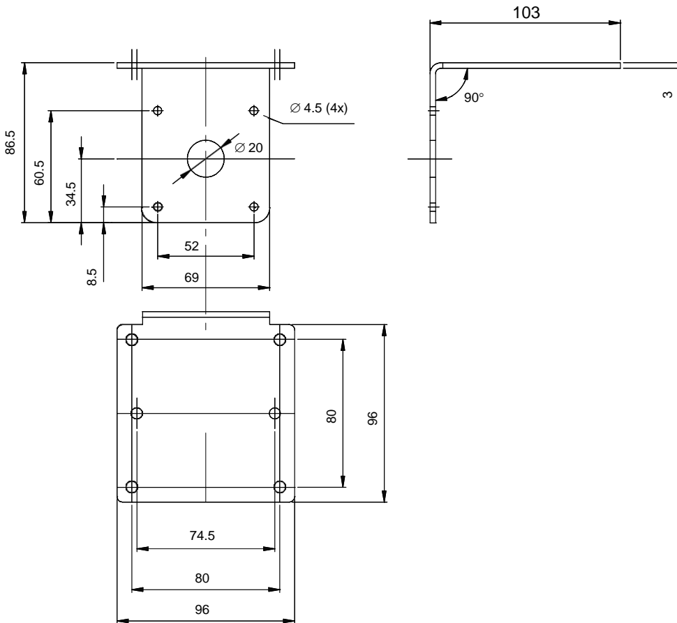
Fig. 8. Mounting bracket A4021A for VQ400 and VE5000 Series in millimeters.
