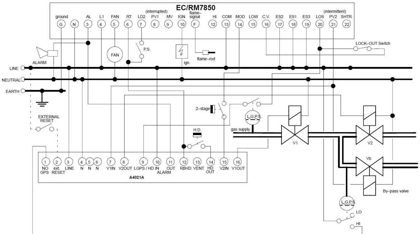
Fig. 17. Wiring diagram A4021A-- EC7850 with by--pass valve, post configuration
