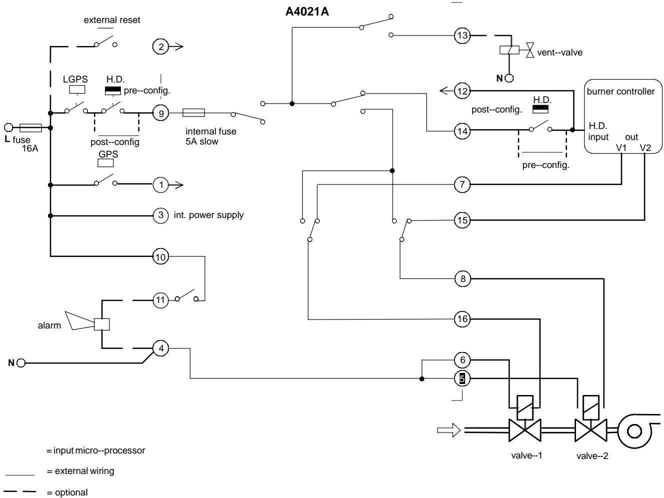
Fig. 9. Simplified internal schematic and wiring diagram pre- and post-test configuration.
