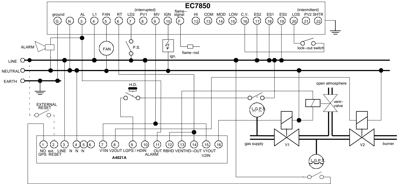
Fig. 14. Wiring diagram A4021A-- EC7850 pre-configuration: intermittent pilot and vent-valve to open atmosphere
