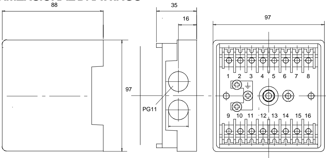
Fig. 7. Mounting dimensions of A4021A and subbase in millimeters
