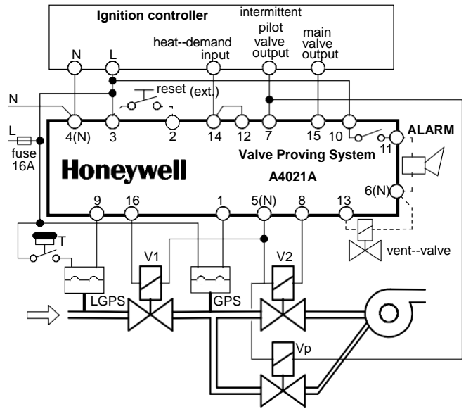
Fig. 12. wiring diagram 3--valve configuration (pre--configuration)
