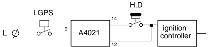
Fig. 3. Valve proving post-configuration .
