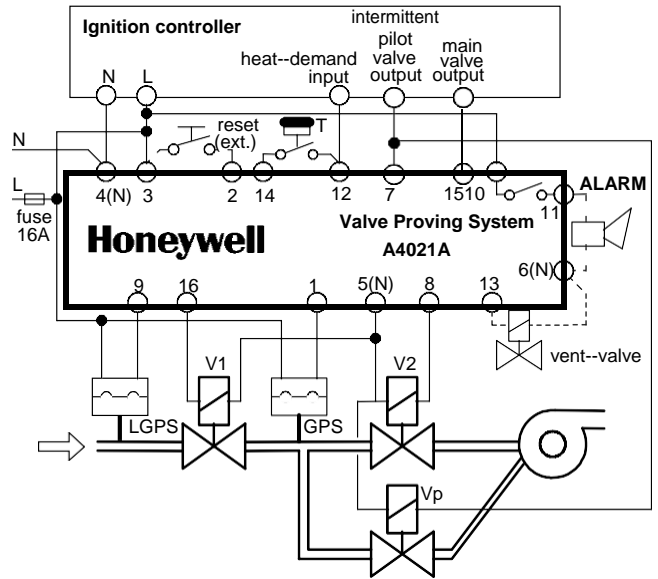
Fig. 13. Wiring diagram 3--valve configuration (post--configuration)
