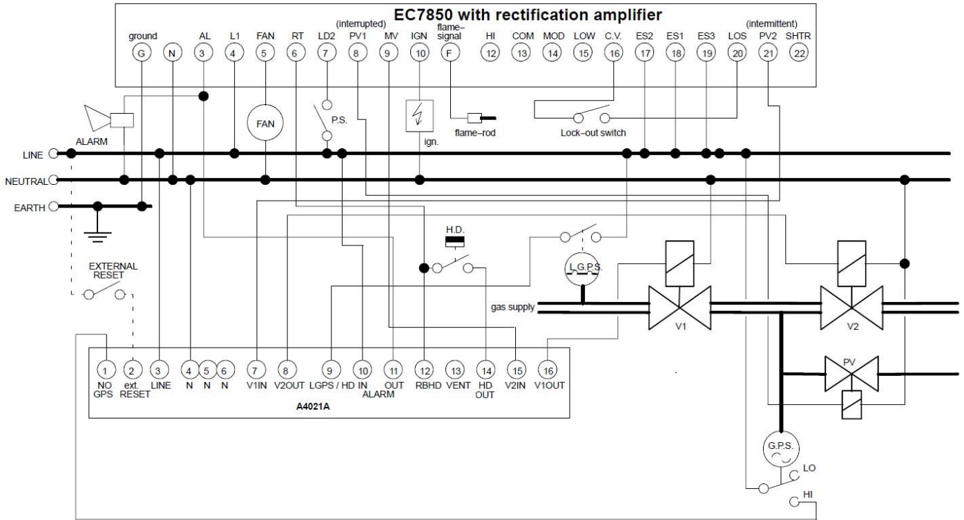
Fig. 16. Wiring diagram A4021A -- EC7850, post--configuration: intermittent system with 3--valve configuration
