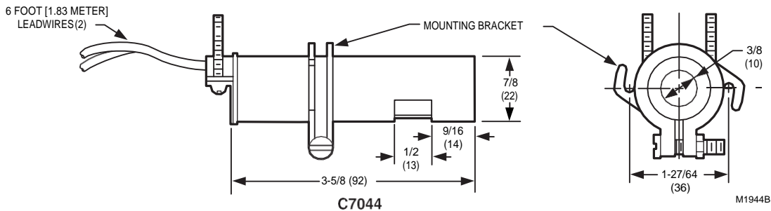
Fig. 3. Installation dimensions of C7044A in in. (mm).
