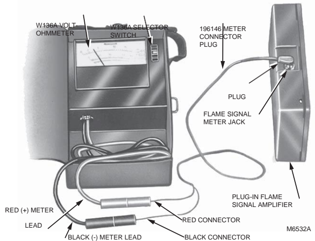
Fig. 10. Measuring microamp flame signal.
