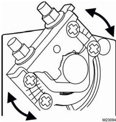
Fig 6. Mechanical endlimits
