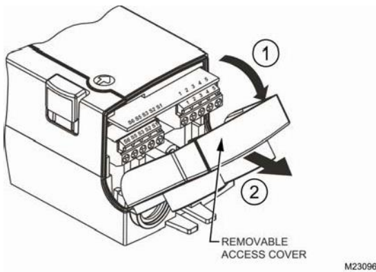
Fig 9. Access Cover
