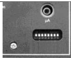
Fig 4-5 Configuration DIP switches (VPS) on the front of the DBC2000E (ENH/ULT only)
