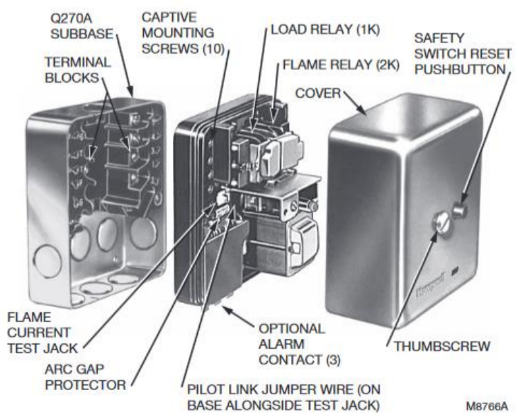
Fig. 6. RA890F and Q270A Subbase.
