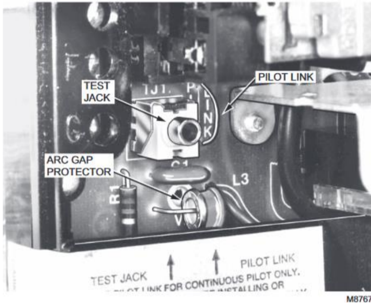
Fig. 7. Location of arc gap protector on RA890F.
