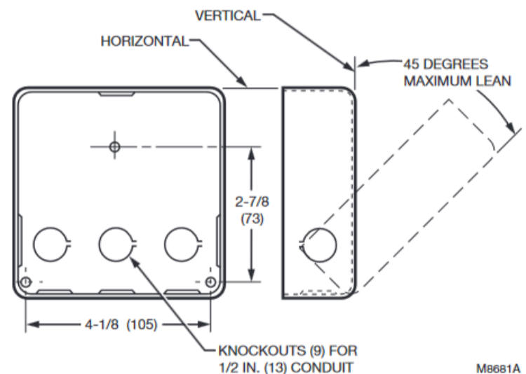
Fig. 1. Mounting subbase in in. (mm).
