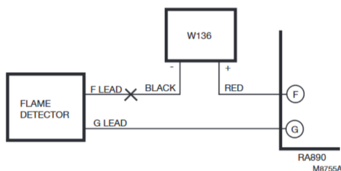
Fig. 8. Connecting meter to read flame current.
