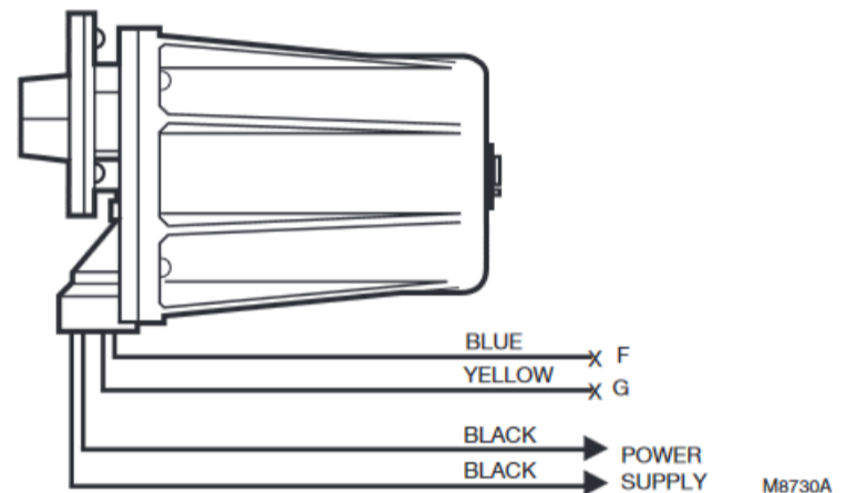
Fig. 2. Flame detector wiring.
