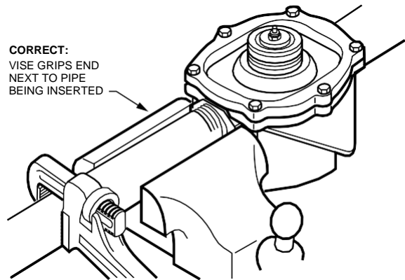
Fig. 5—Installing a 3/4 through 3 in. V5055 Valve.
