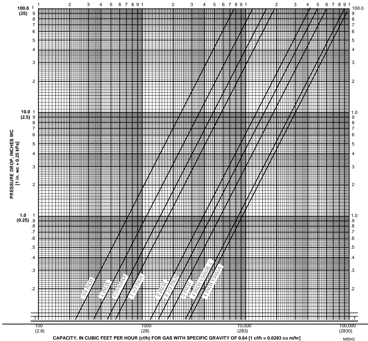
Fig. 1—Flow curves for V5055 Valves.
