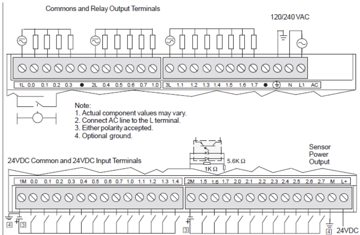
Figure 2 Connector Terminal Identification for CPU 226 AC/DC/Relay
