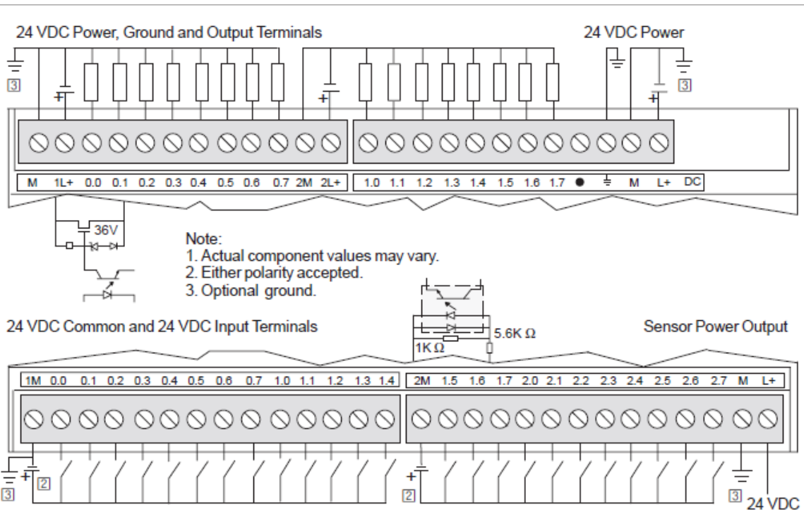
Figure 1 Connector Terminal Identification for CPU 226 DC/DC/DC
