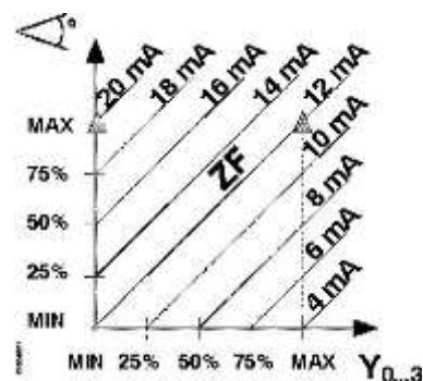
Figure 16. Split Ranging.
