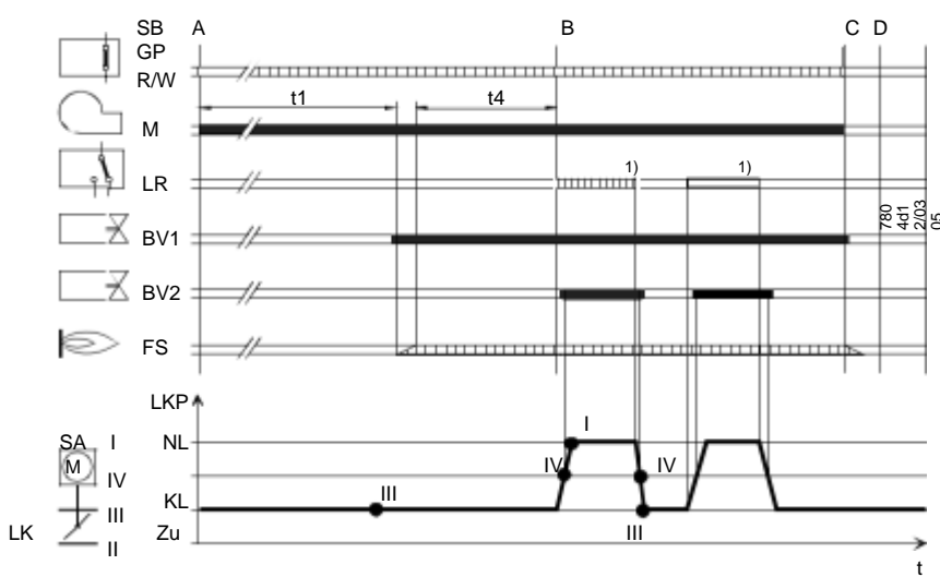
Program sequence without oil preheate
